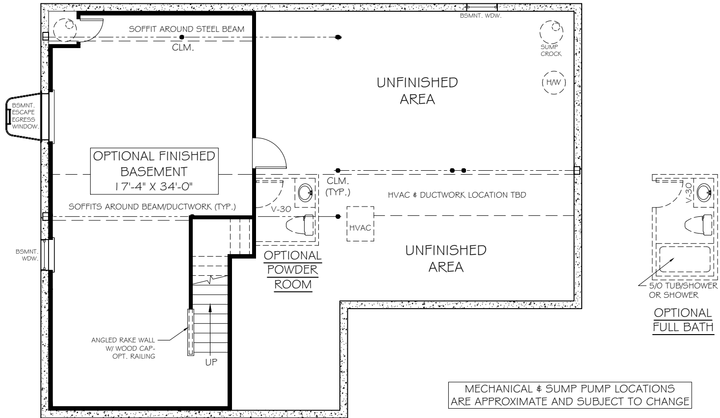
OPTIONAL FINISHED BASEMENT PLAN
