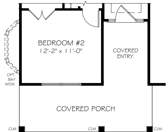
'C' EL. PORCH PLAN
