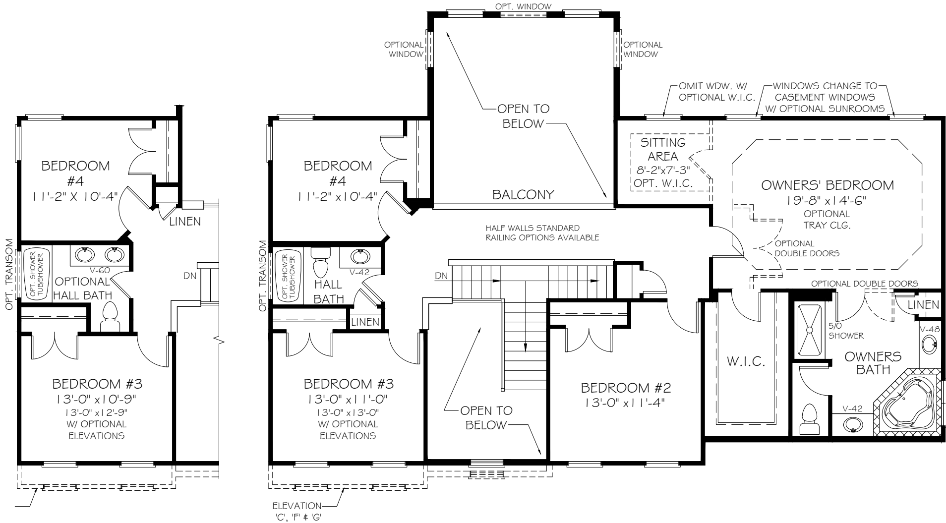
OPTIONAL HALL BATH LAYOUT
