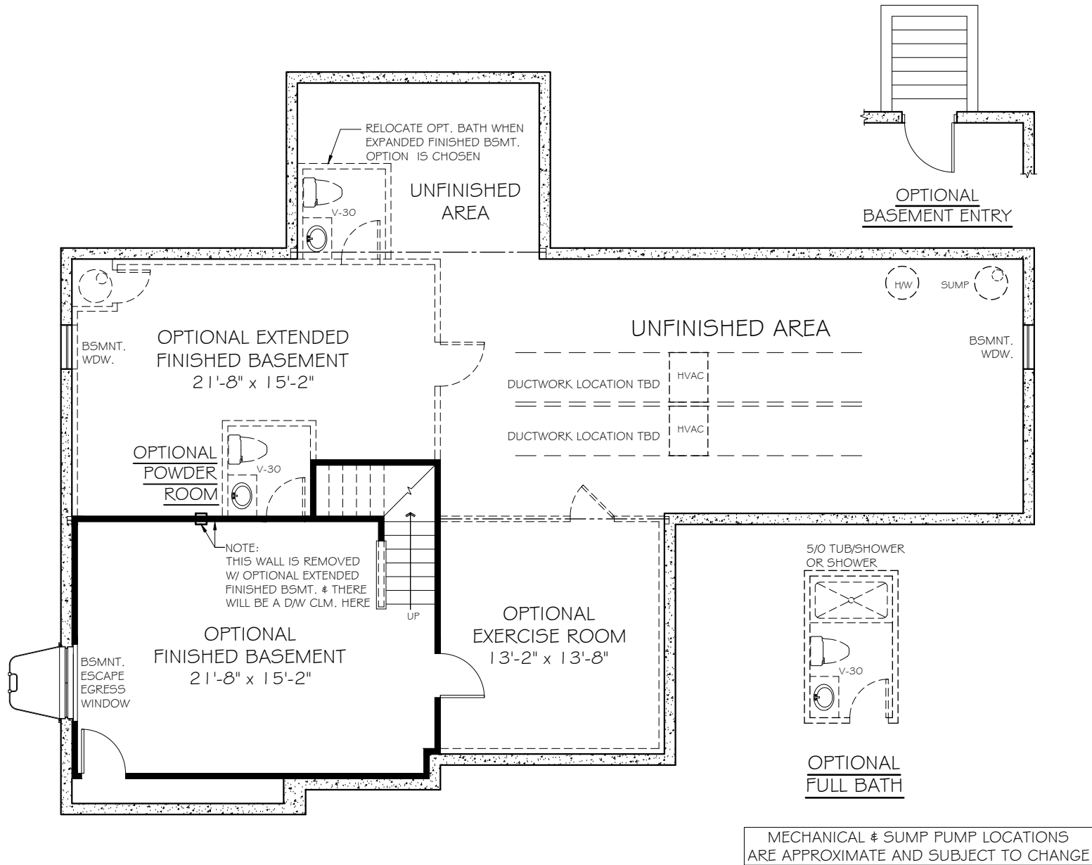
OPTIONAL FINISHED BASEMENT PLAN
