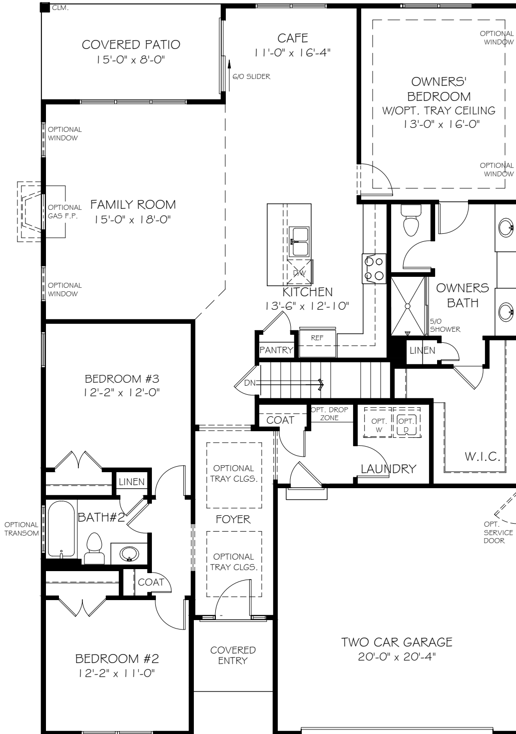
'A' EL. FLOOR PLAN
