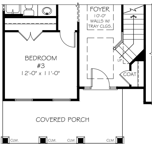
'C' EL. PORCH PLAN
