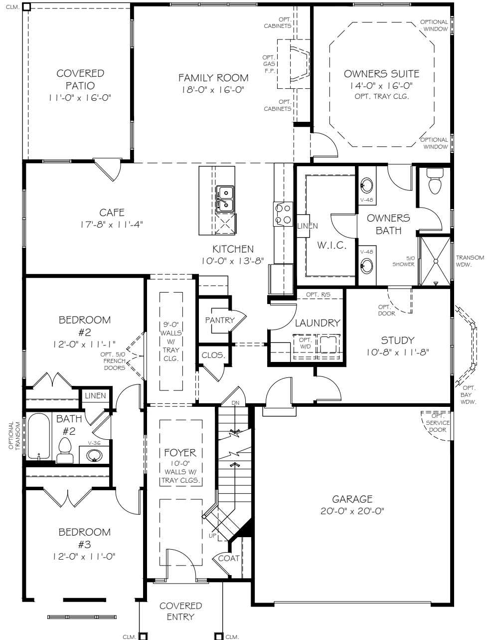
'A' EL. FIRST FLOOR PLAN
