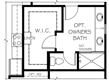
OPTIONAL OWNERS BATH PLAN
