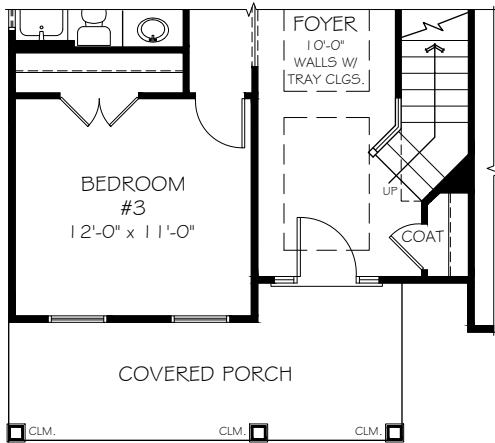
'B' EL. PORCH PLAN
