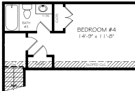
OPT. 2nd FLOOR 4th BED. & BATH
