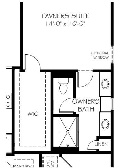
UPGRADED SHOWER OPTION
