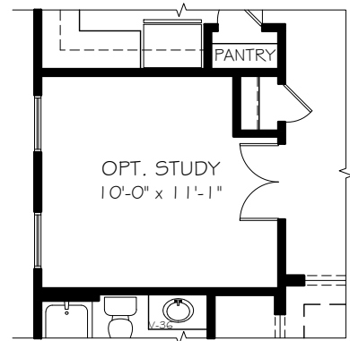
OPTIONAL STUDY LAYOUT
