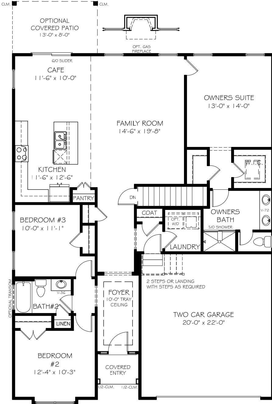
'A' EL. FLOOR PLAN
