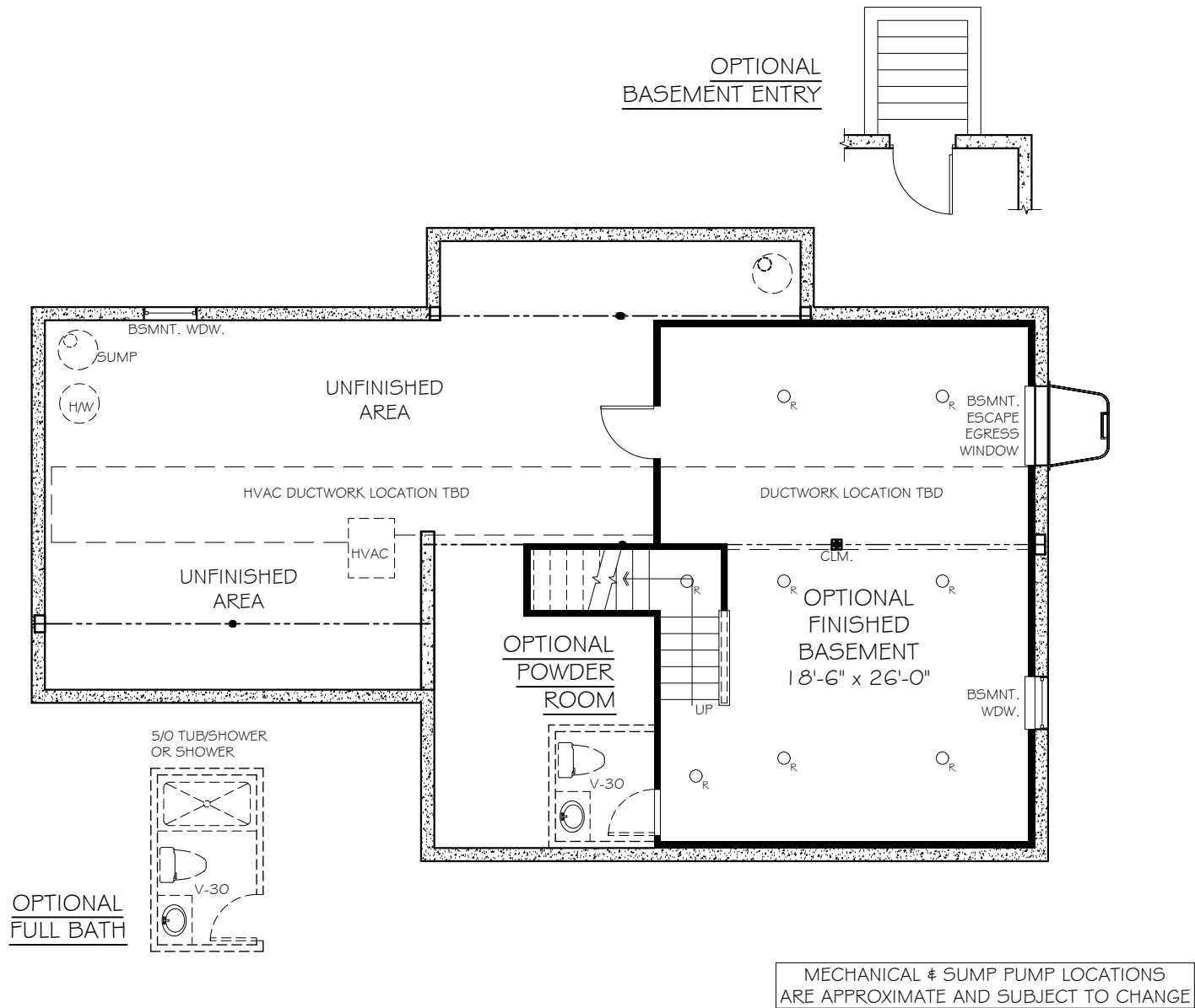
OPTIONAL FINISHED BASEMENT PLAN
